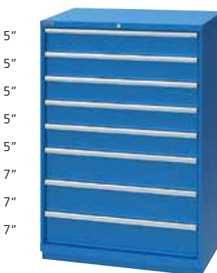
XSHS1350-0801-■□ 40 1/4" W x 22 1/2" D x 59 1/2" H 8 drawers 126 drawer compartments To complete order, include lock and color codes in part number
