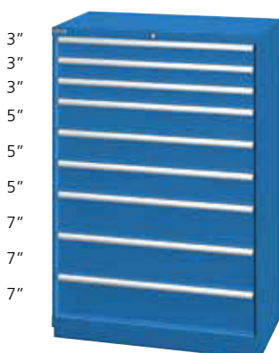
XSHS1350-0902-■□ 40 1/4" W x 22 1/2" D x 59 1/2" H 9 drawers 105 drawer compartments To complete order, include lock and color codes in part number
