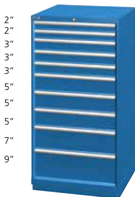
XSSC1350-1002-■□ 28 1/4" W x 28 1/2" D x 59 1/2" H 10 drawers 161 drawer compartments To complete order, include lock and color codes in part number
