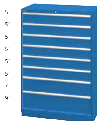
XSHS1350-0803-■□ 40 1/4" W x 22 1/2" D x 59 1/2" H 8 drawers 84 drawer compartments To complete order, include lock and color codes in part number
