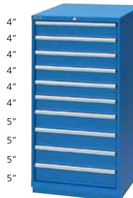
XSSC1350-1017-■□ 28 1/4" W x 28 1/2" D x 59 1/2" H 10 drawers 206 drawer compartments To complete order, include lock and color codes in part number
