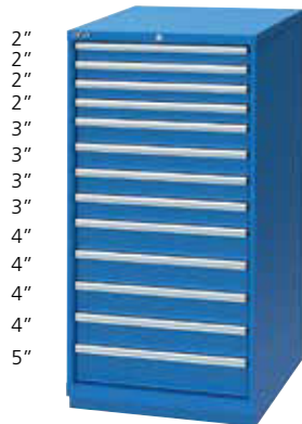
XSSC1350-1320-■□ 28 1/4" W x 28 1/2" D x 59 1/2" H 13 drawers 273 drawer compartments To complete order, include lock and color codes in part number
