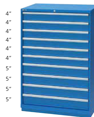
XSHS1350-1017-■□ 40 1/4" W x 22 1/2" D x 59 1/2" H 10 drawers 177 drawer compartments To complete order, include lock and color codes in part number
