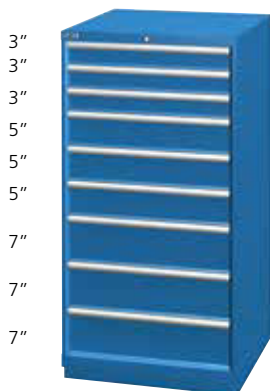
XSSC1350-0902-■□ 28 1/4" W x 28 1/2" D x 59 1/2" H 9 drawers 111 drawer compartments To complete order, include lock and color codes in part number
