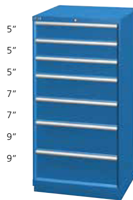
XSSC1350-0702-■□ 28 1/4" W x 28 1/2" D x 59 1/2" H 7 drawers 62 drawer compartments To complete order, include lock and color codes in part number
