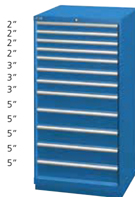
XSSC1350-1234-■□ 28 1/4" W x 28 1/2" D x 59 1/2" H 12 drawers 210 drawer compartments To complete order, include lock and color codes in part number
