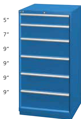
XSSC1350-0608-■□ 28 1/4" W x 28 1/2" D x 59 1/2" H 6 drawers 37 drawer compartments To complete order, include lock and color codes in part number
