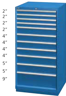
XSSC1350-1103-■□ 28 1/4" W x 28 1/2" D x 59 1/2" H 11 drawers 172 drawer compartments To complete order, include lock and color codes in part number
