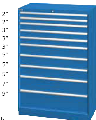
XSHS1350-1002-■□ 40 1/4" W x 22 1/2" D x 59 1/2" H 10 drawers 159 drawer compartments To complete order, include lock and color codes in part number
