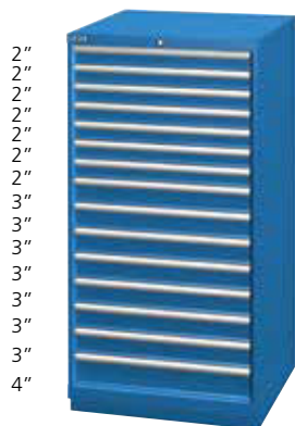
XSSC1350-1502-■□ 28 1/4" W x 28 1/2" D x 59 1/2" H 15 drawers 300 drawer compartments To complete order, include lock and color codes in part number
