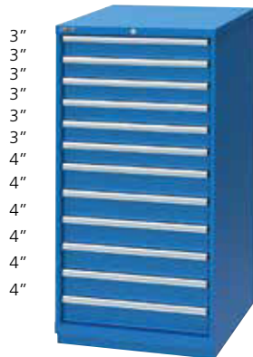
XSSC1350-1233-■□ 28 1/4" W x 28 1/2" D x 59 1/2" H 12 drawers 264 drawer compartments To complete order, include lock and color codes in part number
