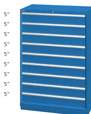
XSHS1350-0903-■□ 40 1/4" W x 22 1/2" D x 59 1/2" H 9 drawers 120 drawer compartments To complete order, include lock and color codes in part number
