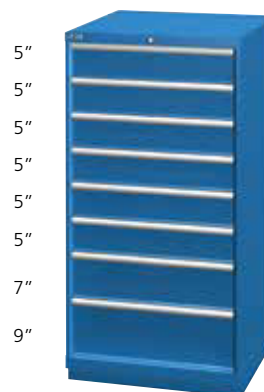
XSSC1350-0803-■□ 28 1/4" W x 28 1/2" D x 59 1/2" H 8 drawers 88 drawer compartments To complete order, include lock and color codes in part number
