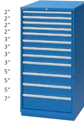
XSSC1350-1201-■□ 28 1/4" W x 28 1/2" D x 59 1/2" H 12 drawers 245 drawer compartments To complete order, include lock and color codes in part number
