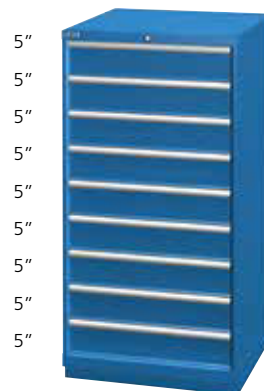
XSSC1350-0903-■□ 28 1/4" W x 28 1/2" D x 59 1/2" H 9 drawers 124 drawer compartments To complete order, include lock and color codes in part number
