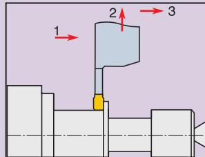
Roughing (correct)
