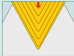
Radial Infeed
