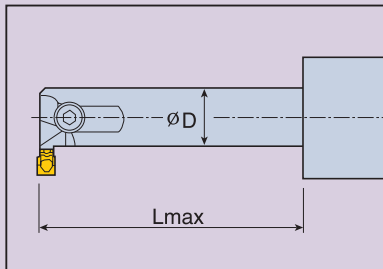
Toolholder Overhang
