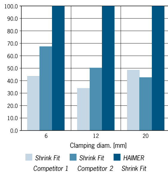
Clamping torque, percentage (HAIMER = 100%)
