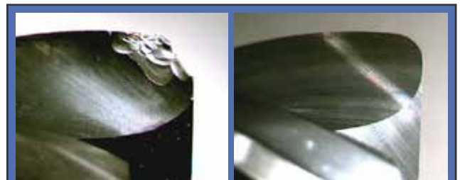
This end mill arrived with heavy chipping on the flute end (left). Guhring Reconditioning restored a correct cutting edge (right). The result: Greatly extended tool life and significant cost savings.
